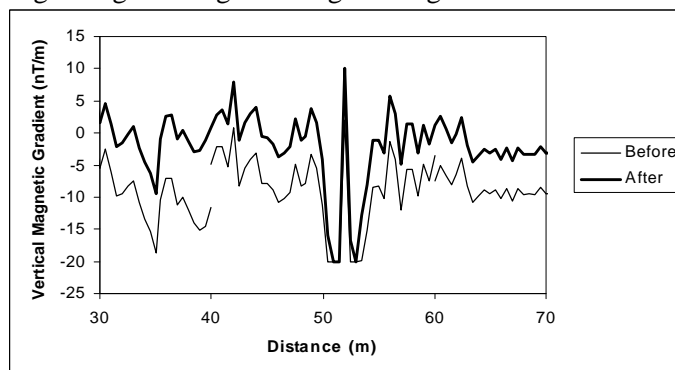
Figure 3. Profile AA' (position shown in Figure 1) before and after merging. Amplitudes have been clipped to 20nT/km.
