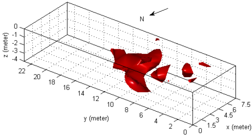
FIG. 7. Iso-resistivity surface of the highest resistivity zones ( > 2.7 \log \text{ ohm.m} ).
