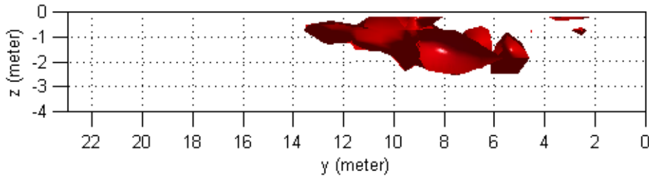
FIG. 8. The cross-section of the iso-resistivity surface ( > 2.7 \log \text{ ohm.m} ).
