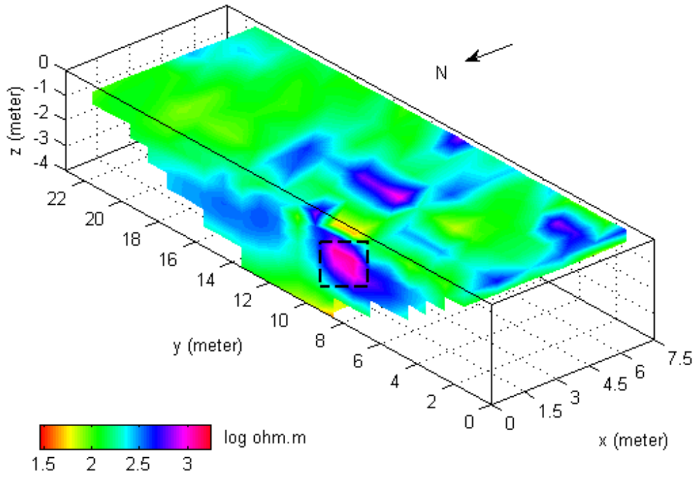
FIG. 5. Pseudo three-dimensional geo-electrical model of the investigation area. The high resistivity anomaly (black rectangle) is related to a man-made structure.
