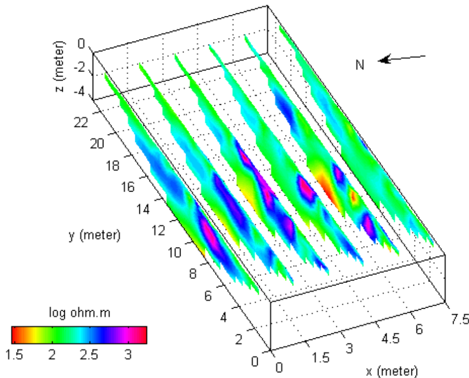
FIG. 4. Two-dimensional geo-electrical sections of the six profiles. Profiles 1 and 6 are located at 0 m and 7.5 m along x-axis, respectively.
