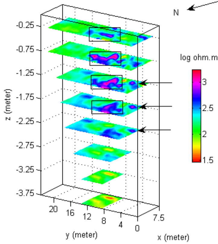
FIG. 6. Horizontal slices of the pseudo three-dimensional resistivity distribution with 0.5 m depth interval. The high resistivity anomalies, marked with rectangles and arrows, are related to man-made structures.
