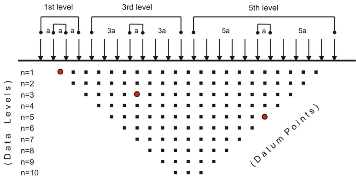
FIG. 2. Sequence of measurements to create a pseudo-section using Wenner-Schlumberger array. The datum points and the data levels are displayed.
